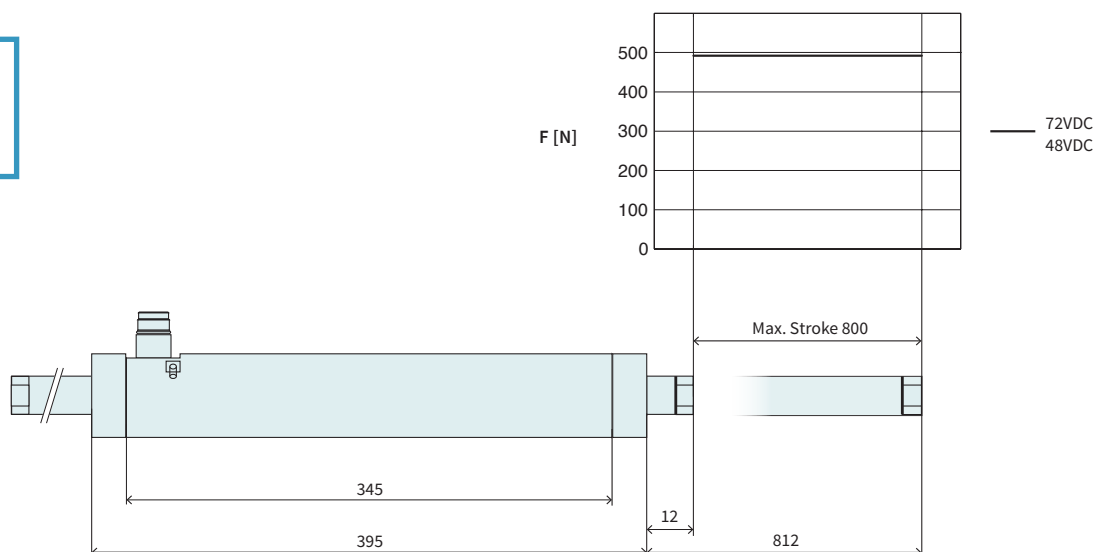
Technical Data P01-48x240F/800x800-EX-E
