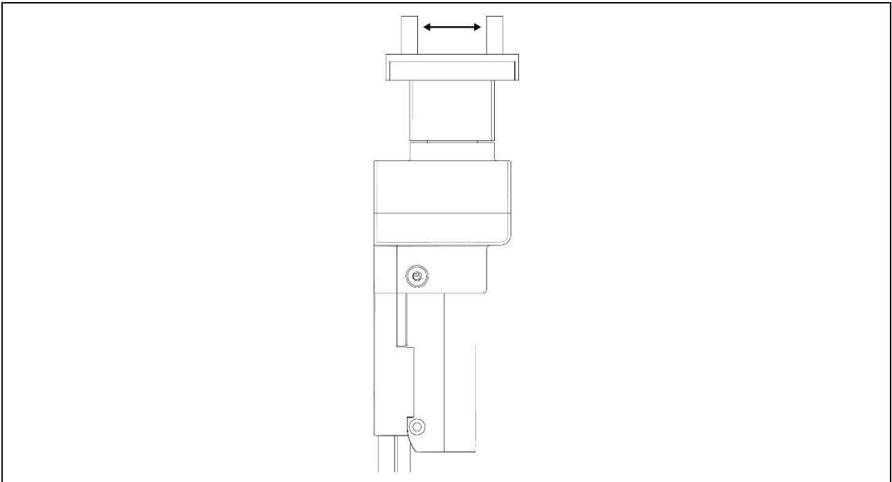
Example 2: vertical mounting with a "gripper at the top". This is used for gripping, placing, mounting, separating, spreading, aligning and centring products.
