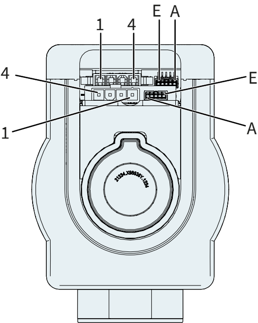
View: motor connector, plug side Top: NG-connector rotary motor Bottom: N-connector linear motor
