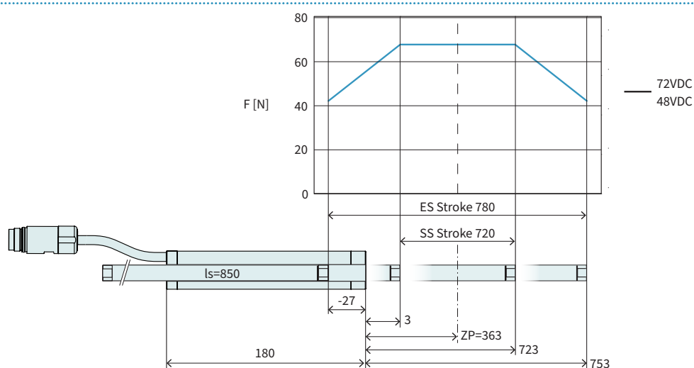
Technical Data P01-23x80F/720x780-HP-SSCP
