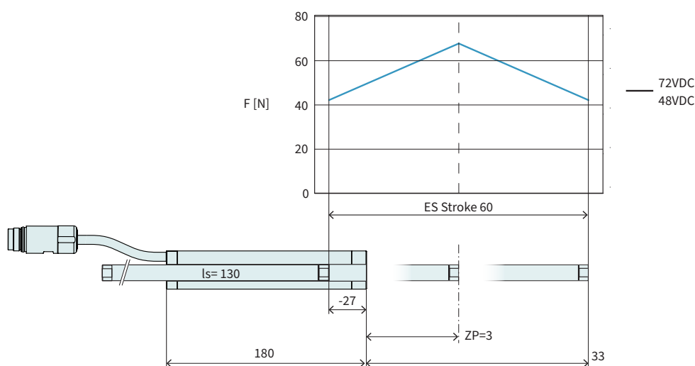
Technical Data P01-23x80F/0x60-HP-SSCP
