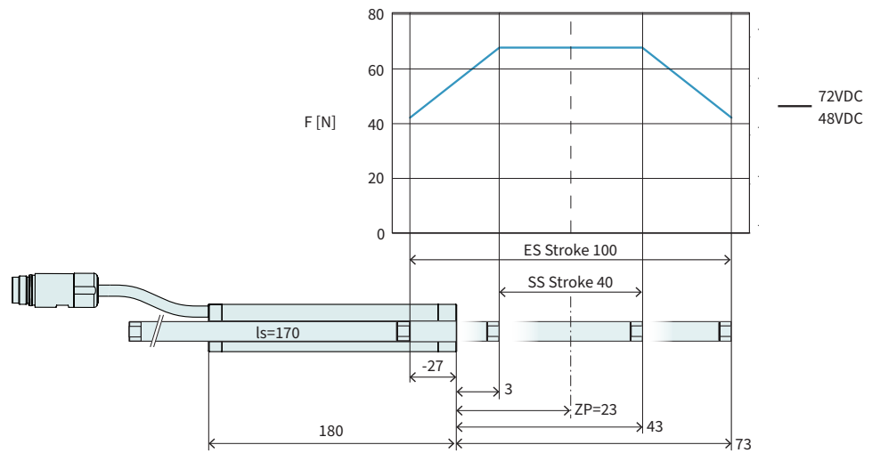
Technical Data P01-23x80F/40x100-HP-SSCP
