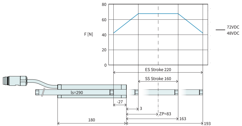
Technical Data P01-23x80F/160x220-HP-SSCP
