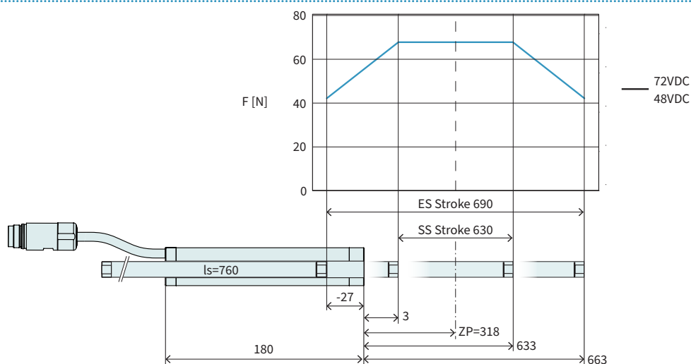
Technical Data P01-23x80F/630x690-HP-SSCP
