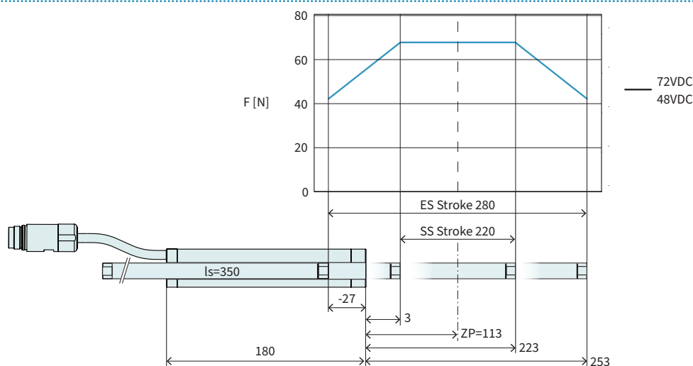
Technical Data P01-23x80F/220x280-HP-SSCP
