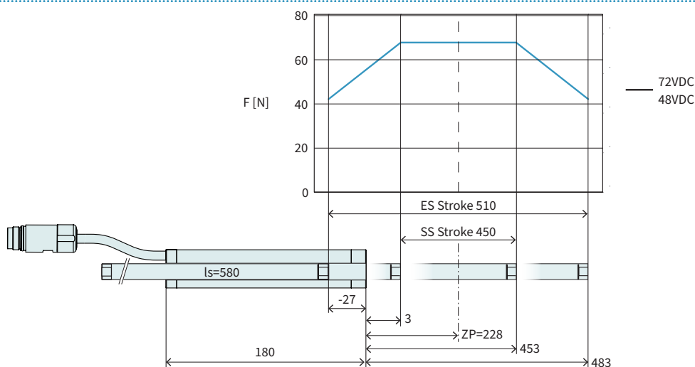
Technical Data P01-23x80F/450x510-HP-SSCP
