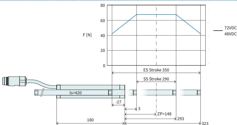
Technical Data P01-23x80F/290x350-HP-SSCP
