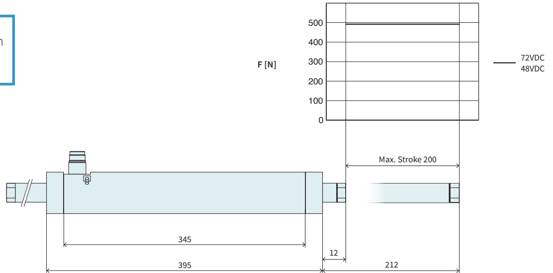
Technical Data P01-48x240F/200x200-HP-EX-E
