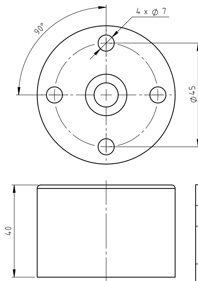
0150-4500 Z01-SF-30-SSC Adapter dimensions
